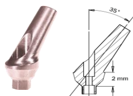
Angular Abutment 35°
