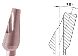
Angular Abutment 15°
